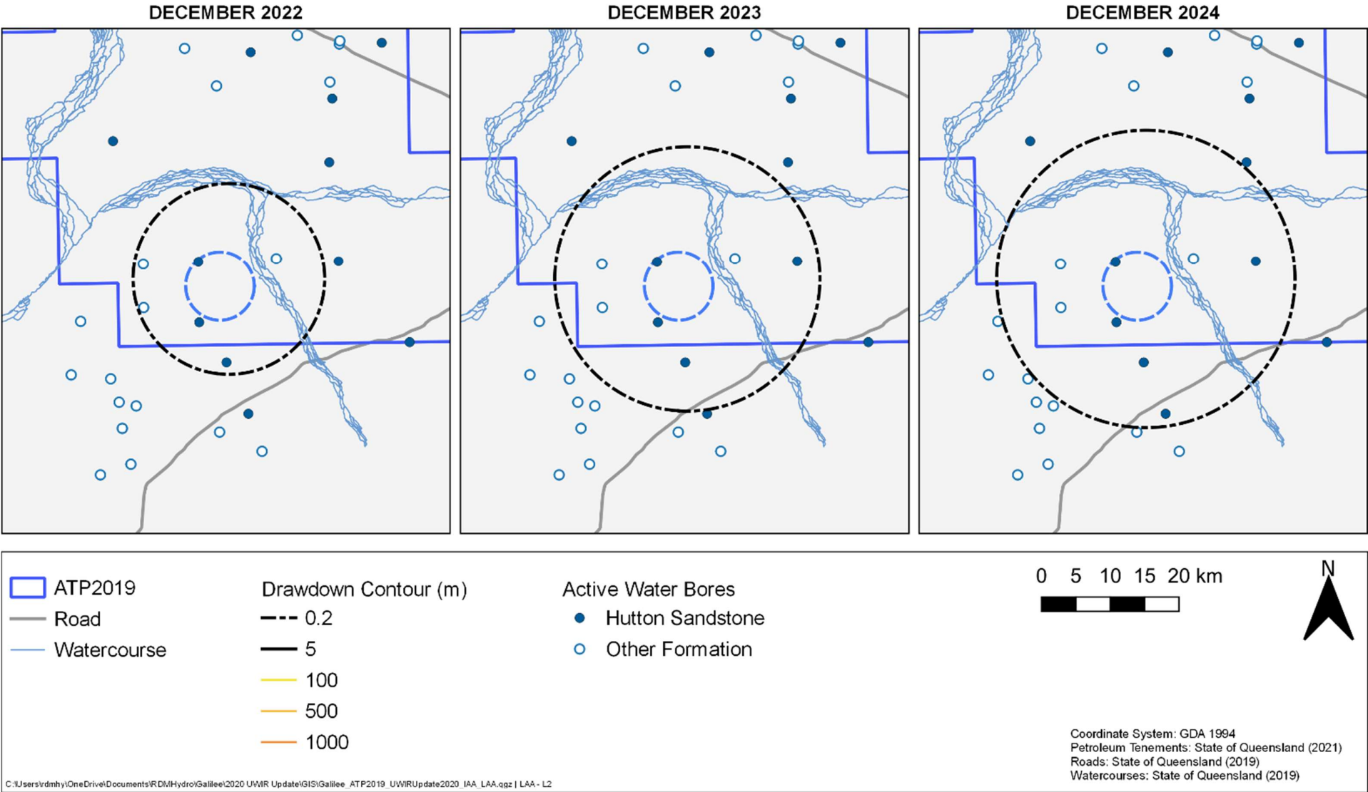
Figure 30 Hutton Sandstone drawdown contours
