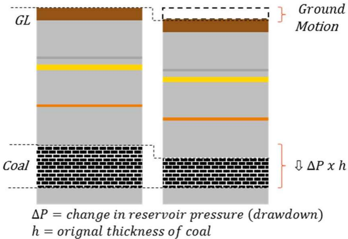
Figure 27 Diagrammatic (not to scale) representation of linear elastic theory to estimate the magnitude of subsidence (APLNG, 2018)
