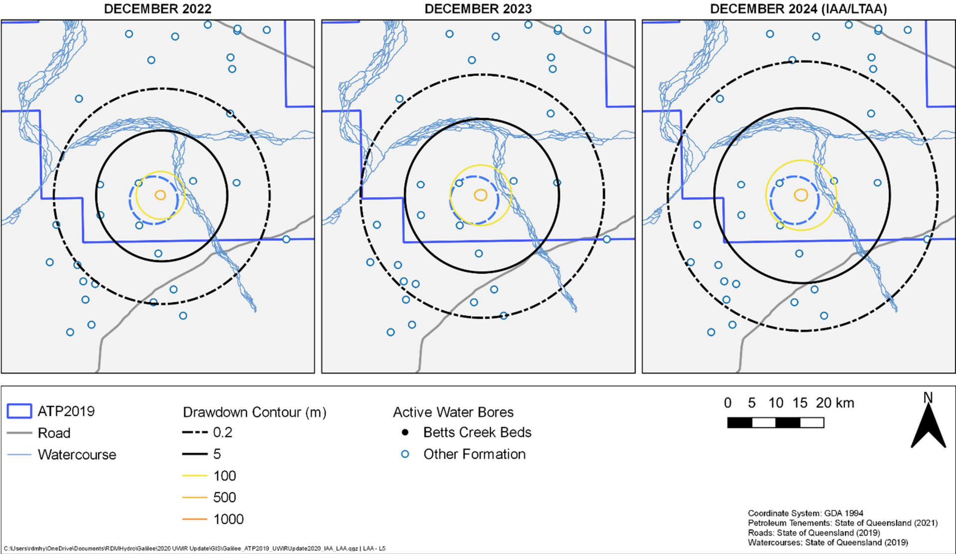
Figure 28 Lower Betts Creek Beds drawdown contours
