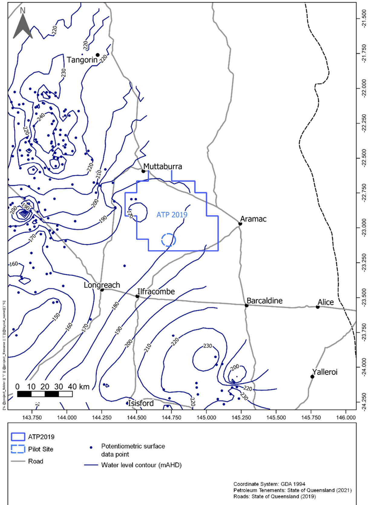
Figure 8 Winton/Mackunda Formations - potentiometric surface
