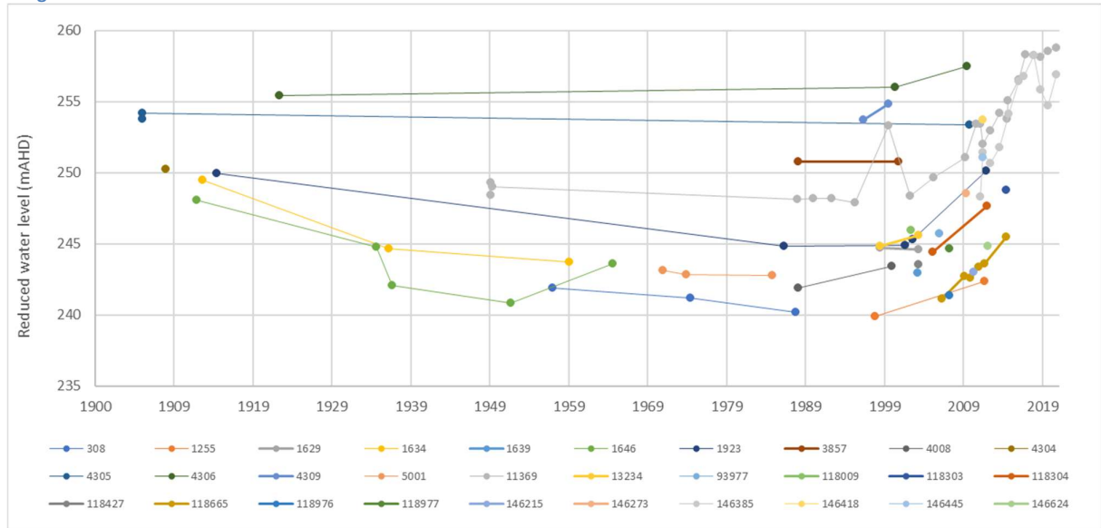
Figure 14 Hutton Sandstone - timeseries water level measurements
