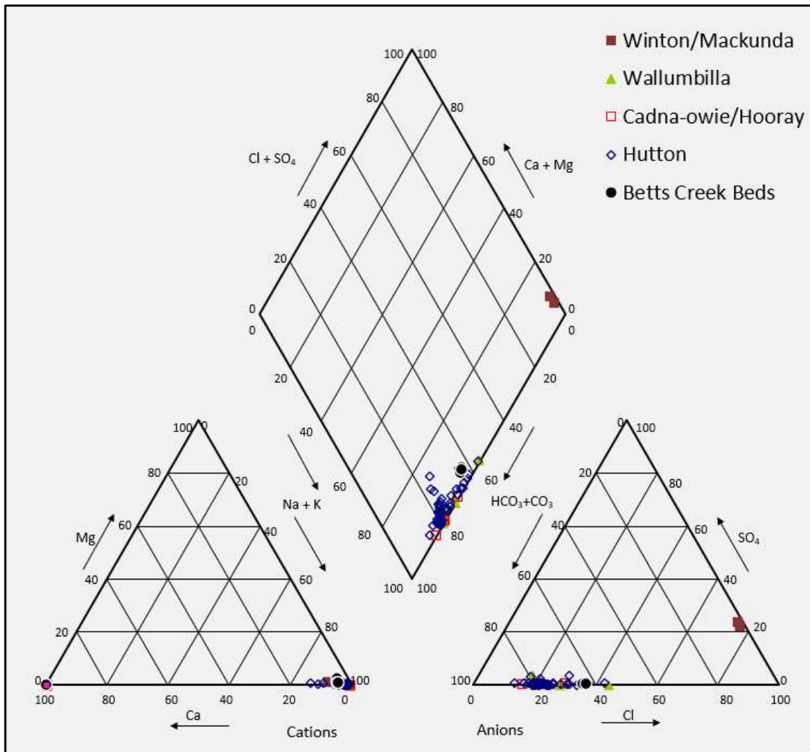
Figure 16 Trilinear plot for water quality data from bores within ATP 2019
