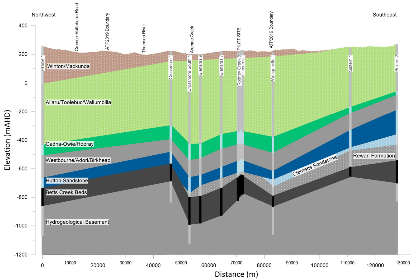
Figure 7 Hydrostratigraphic cross-section through the Pilot Site
