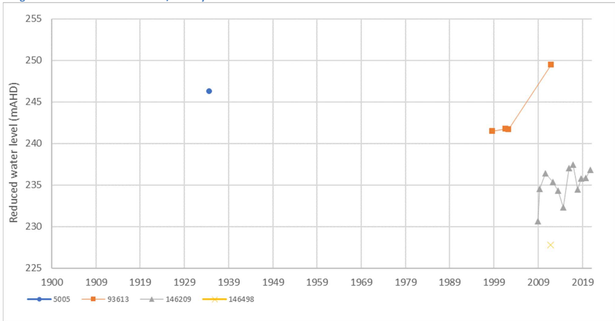
Figure 13 Cadna-owie Formation/Hooray Sandstone - timeseries water level measurements
