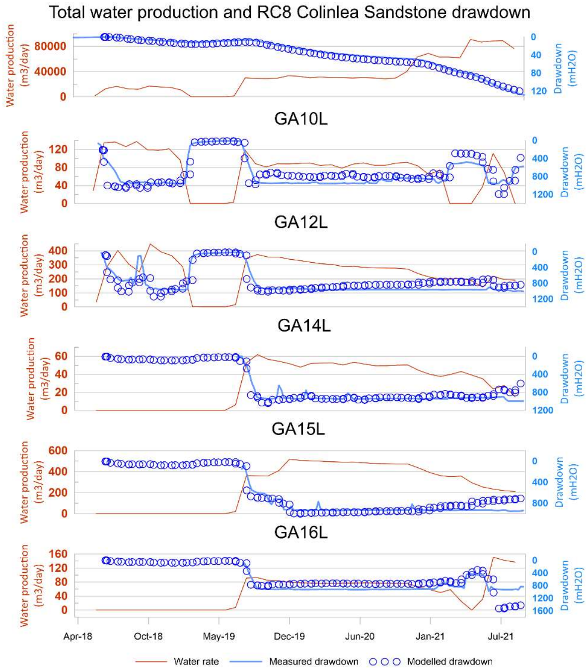
Figure 25 Multi-lateral Pilot - flow rates with measured and modelled drawdowns (Colinlea Sandstone and lateral wells)
