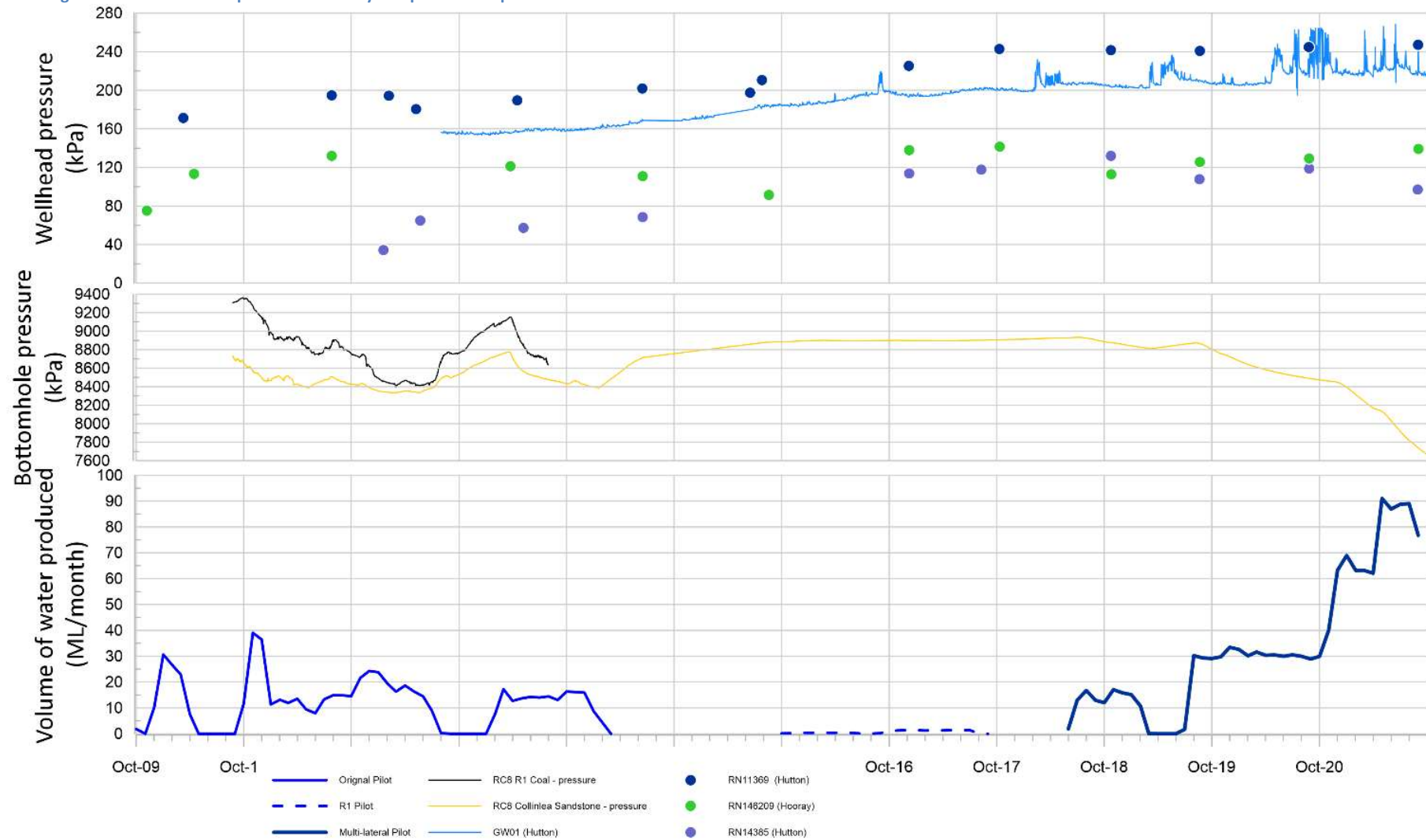
Figure 24 ATP2019 water production history and pressure responses
