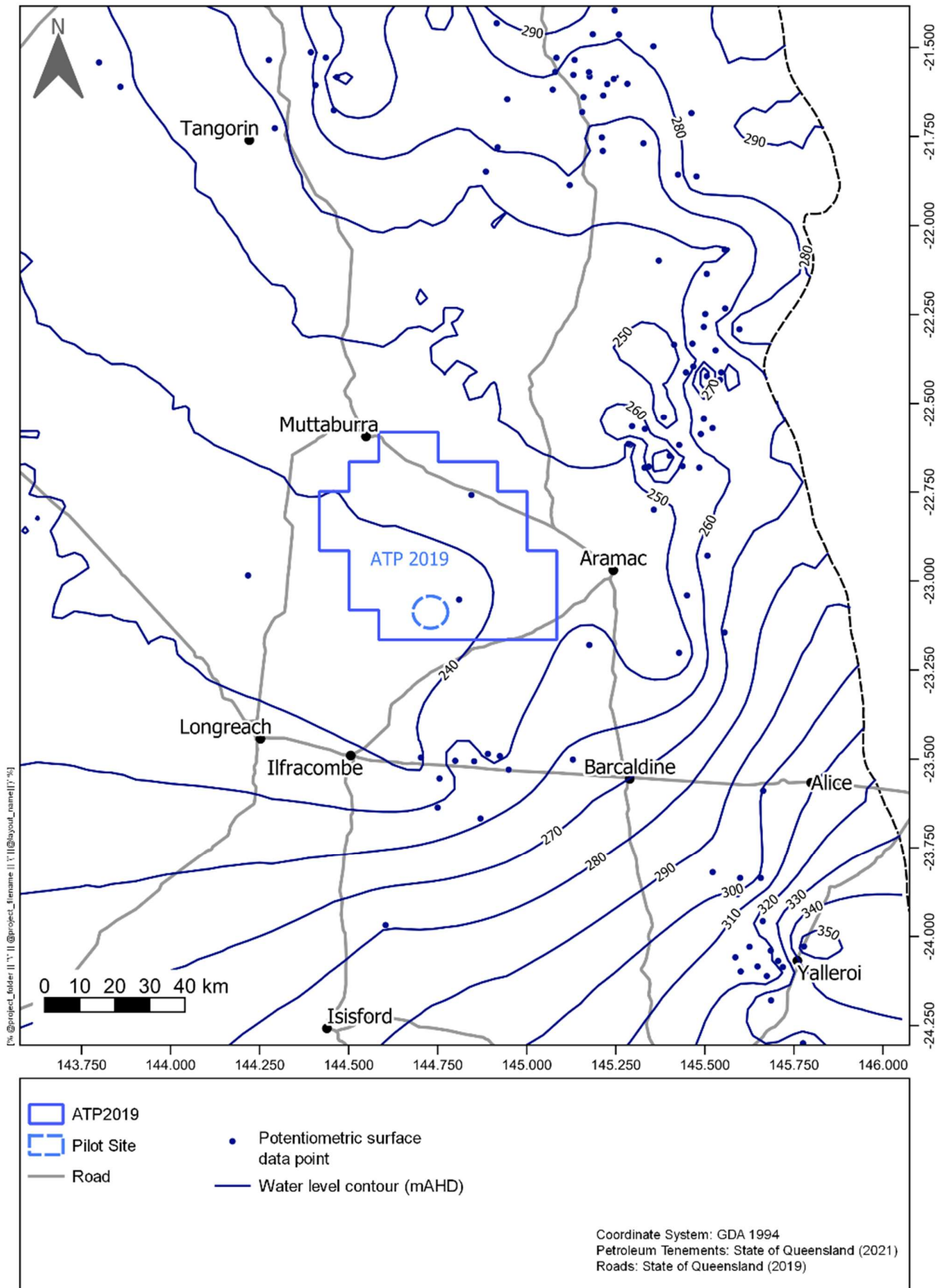
Figure 9 Cadna-owie Formation/Hooray Sandstones - potentiometric surface
