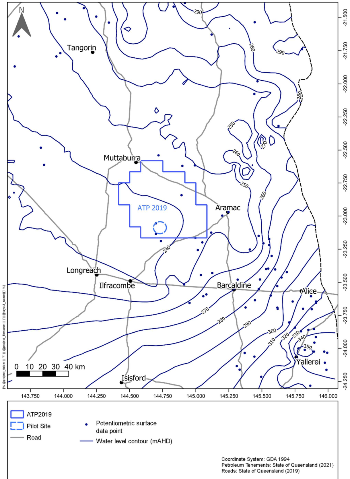
Figure 10 Hutton Sandstone - potentiometric surface
