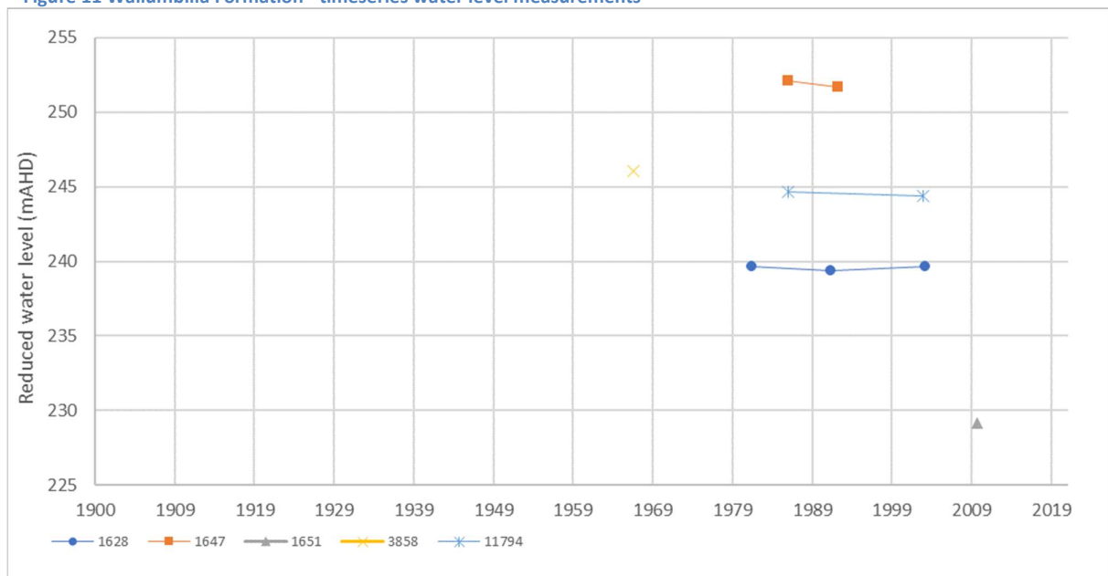
Figure 11 Wallumbilla Formation - timeseries water level measurements
