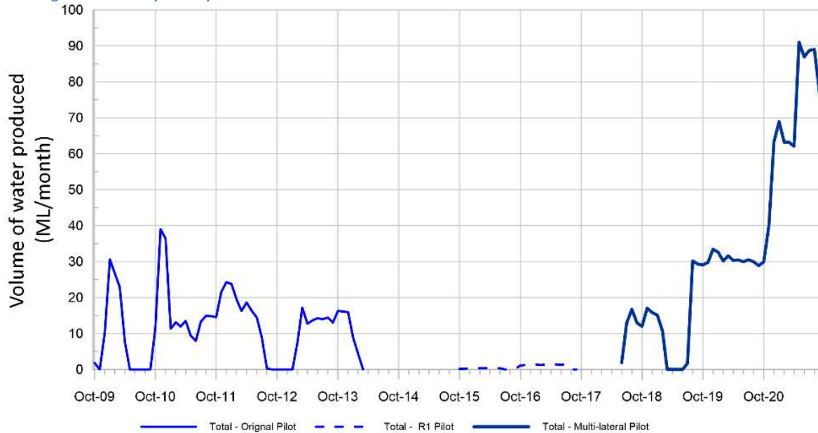
Figure 22 Monthly water production totals
