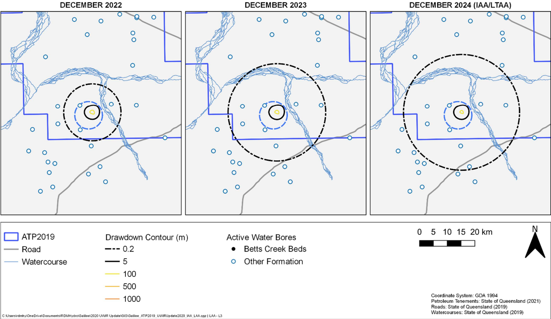
Figure 29 Upper Betts Creek Beds drawdown contours
