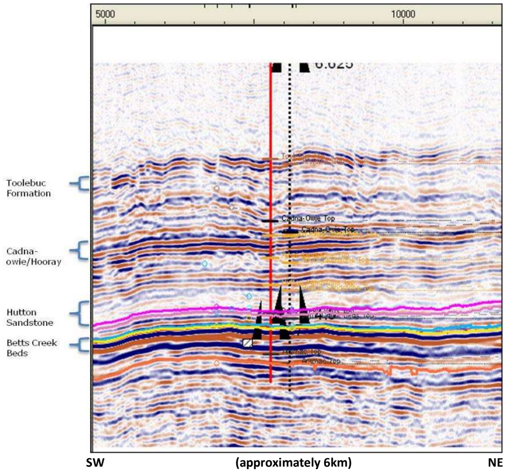
Figure 4 Northeast striking seismic line showing Glenaras Anticline (Sardine SS Line 9)
