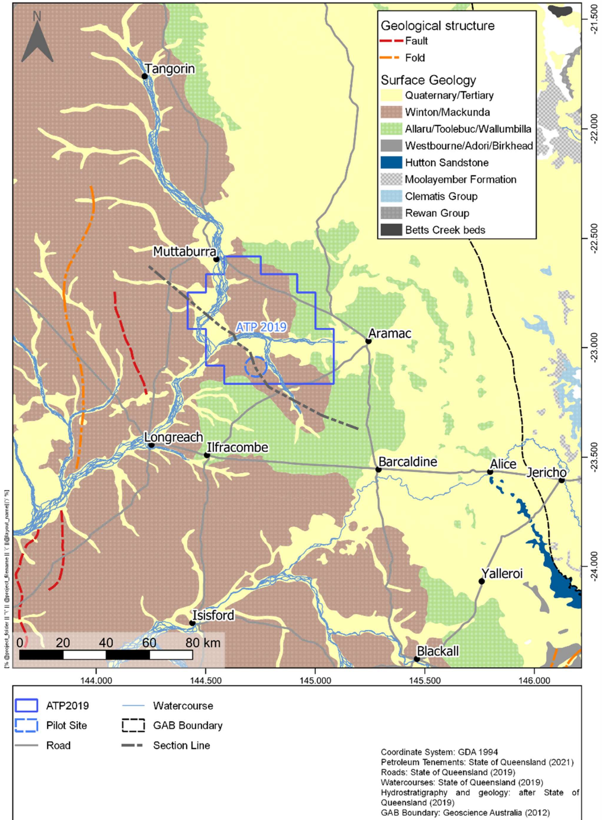
Figure 6 Surface geology simplified into hydrostratigraphic units
